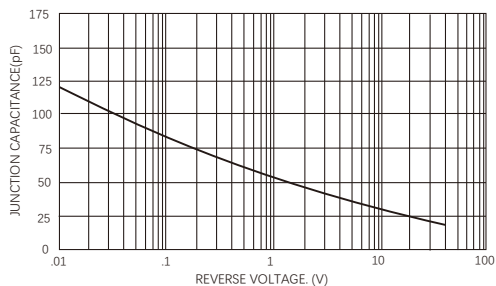
FIG.5-TYPICAL JUNCTION CAPACITANCE
